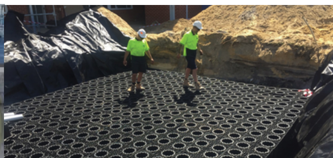
MONOBLOCK CHANNEL
