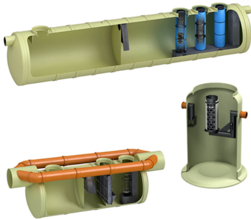
OIL SEPARATOR
